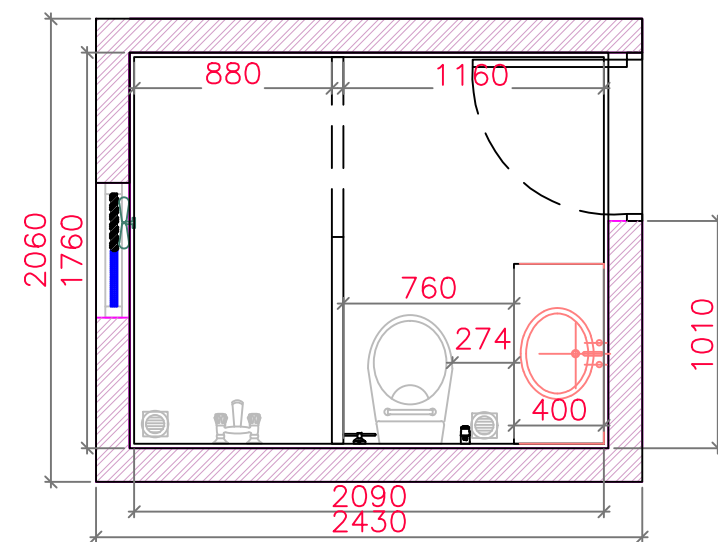
TOILET: FIXTURES LAYOUT
